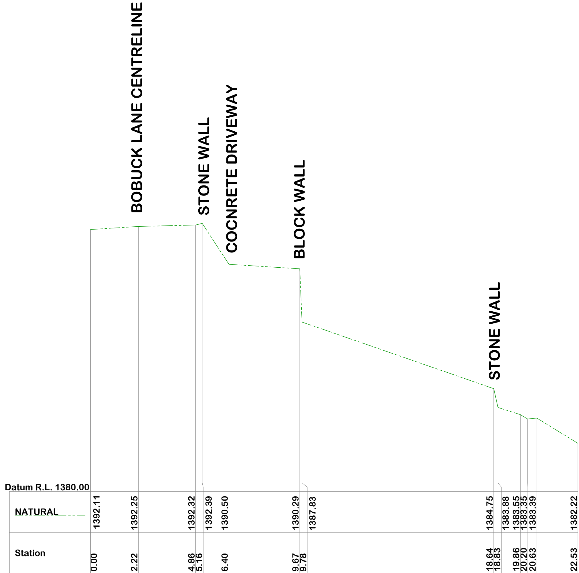
SECTION A - GROUND PROFILE LONG SECTION
